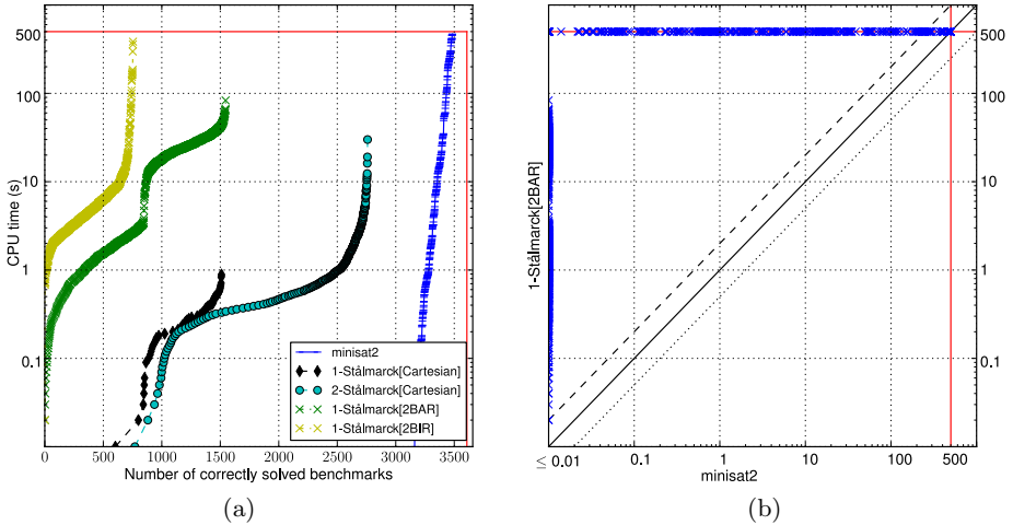
Fig. 12. (a) Semi-log plot showing the number of benchmarks that were each solved correctly in no more than t seconds. (b) Log-log scatter plot of the time taken (in seconds) by MiniSat versus 1\text{-Stålmarck}[\text{2-BAR}] .
