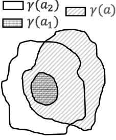
Fig. 2. Abstract Consequence: For all a_1, a_2 \in \mathcal{A} where \gamma(a_1) \subsetneq \gamma(a_2) , if a = \text{AbstractConsequence}(a_1, a_2) , then \gamma(a_1) \subseteq \gamma(a_2) and \gamma(a) \not\supseteq \gamma(a_2)
