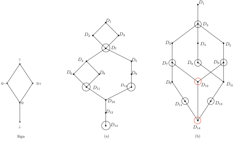
Fig. 2. Lifted lco(\text{Sign})
