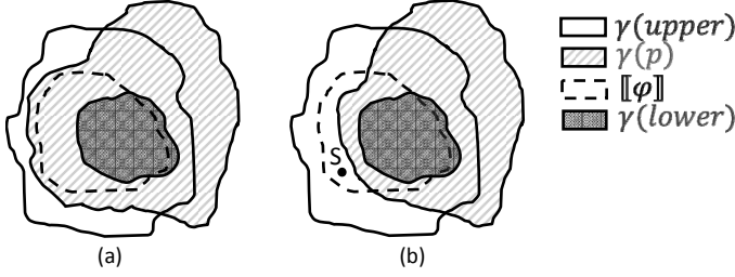
Fig. 3. The two cases arising in Alg. 5: \varphi \wedge \neg \hat{\gamma}(p) is either (a) unsatisfiable, or (b) satisfiable with S \models \varphi and S \not\models \hat{\gamma}(p) . (Note that although lower \sqsubseteq \hat{\alpha}(\varphi) \sqsubseteq upper and \llbracket \varphi \rrbracket \subseteq \gamma(upper) are invariants of Alg. 5, \gamma(lower) \subseteq \llbracket \varphi \rrbracket does not necessarily hold, as depicted above.)
