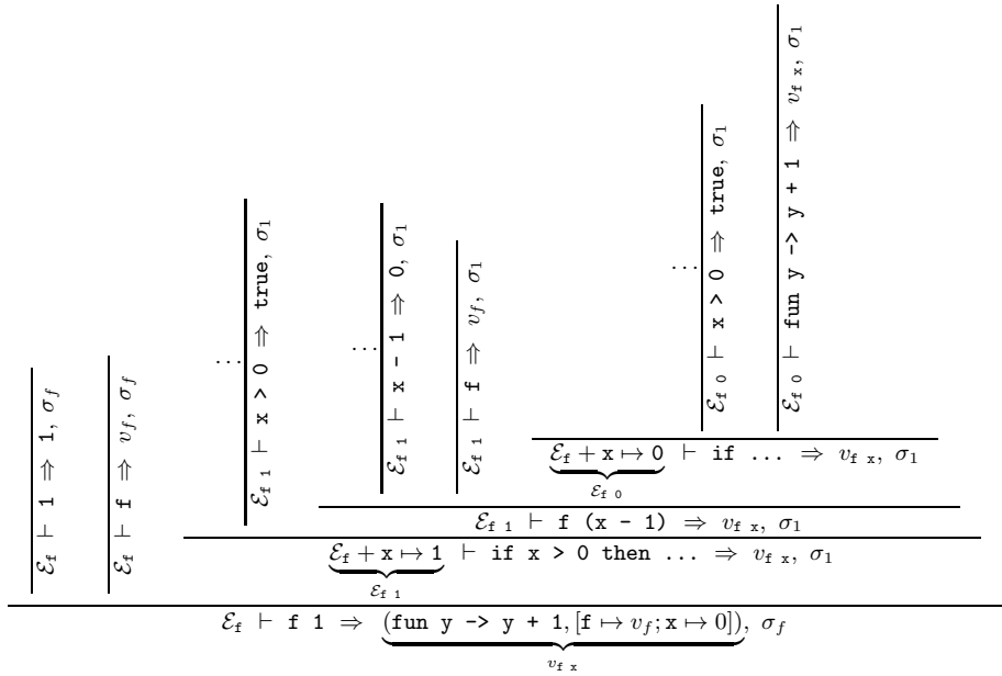
Fig. 2. Annotation of the evaluation tree for f 1 in the environment \mathcal{E}_t = (\mathbf{f}, \text{fun } x \rightarrow \text{if } x > 0 \text{ then } \mathbf{f} \ (x - 1) \text{ else fun } y \rightarrow y + 1, \emptyset) . The initial judgement is annotated with \sigma_f = (\text{false}, 0) . The annotation changes from \sigma_f to \sigma_1 = (\text{true}, 1) after the first call to f . Due to the lack of width, we had to rotate several judgements.
