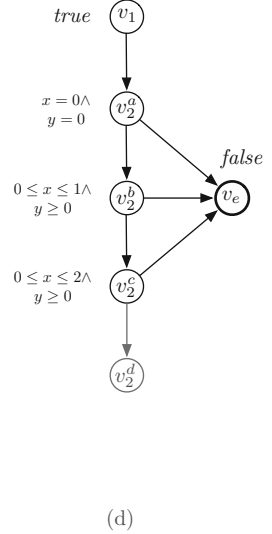
Fig. 2. (a) A safe program P ('*' denotes a nondeterministic choice). (b) A cutpoint graph of P . An ARG of P after (c) the first and (d) after the second AI step.
