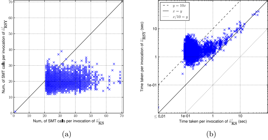
Fig. 1. (a) Scatter plot showing the number of decision-procedure queries during each pair of invocations of \hat{\alpha}_{RSY}^\uparrow and \hat{\alpha}_{KS}^\uparrow , when neither invocation had a decision-procedure timeout. (b) Log-log scatter plot showing the times taken by each pair of invocations of \hat{\alpha}_{RSY}^\uparrow and \hat{\alpha}_{KS}^\uparrow , when neither invocation had a decision-procedure timeout.
