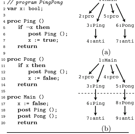
Fig. 6. The PingPong program, along with asynchronous executions of the translations ((\text{PingPong}))_{nt} (a) and ((\text{PingPong-mod2}))_{nt} (b). Task order is indicated by numeric prefixes; the dotted line indicates delaying.
